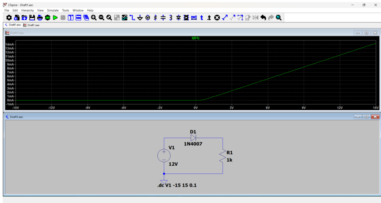
Figure 2: Diode Selection for a Real Application
